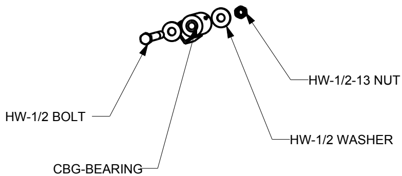
DETAIL C SCALE 7/50
