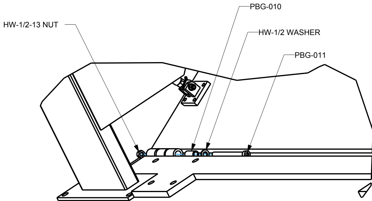
DETAIL D SCALE 3/20
